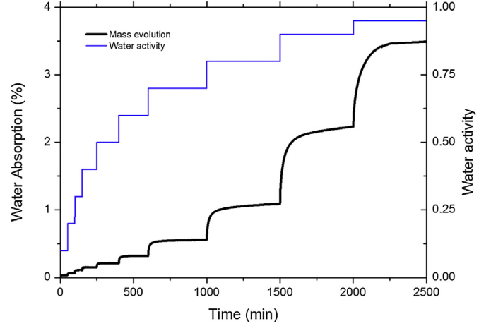
Fig. 5. Water absorption in 100 µm thick film for several water activities at 40 °C.
