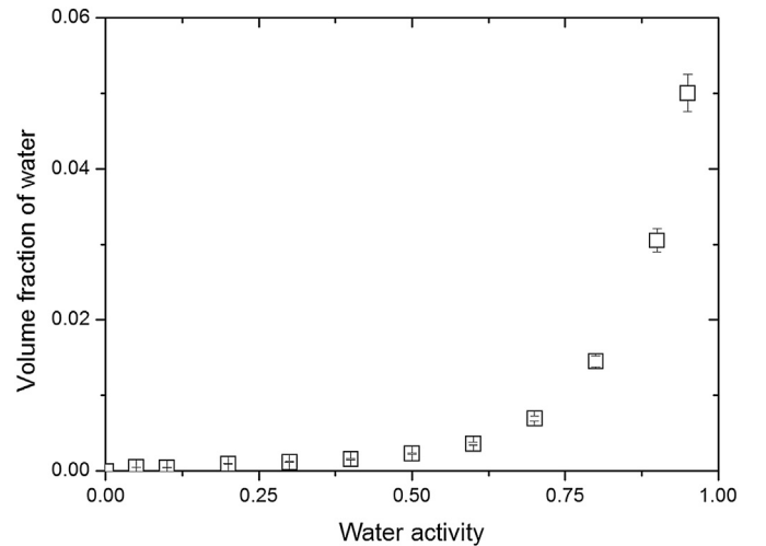
Fig. 6. Volume fraction of water in 100 µm CR film at 40 °C for different water activities.
