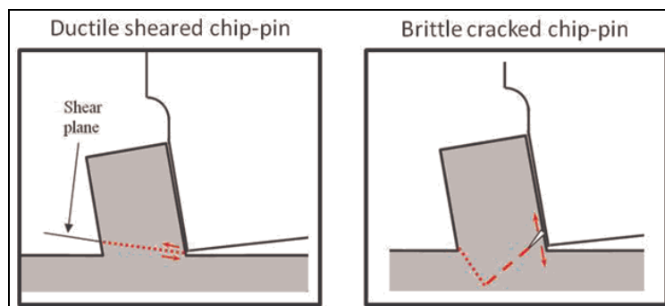
Figure 4- Fracture mechanisms for a negative rake angle of the tool (from [1])
