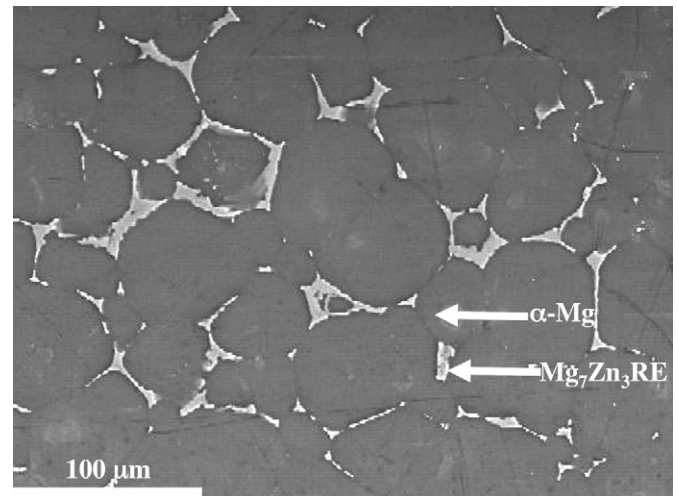
Fig. 1. Scanning electron micrograph of ZE41-T5.
