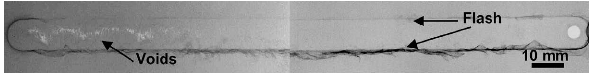
Fig. 5. Radiography of AZ31 welds V = 200 \text{ mm min}^{-1} , W = 800\text{--}1400 \text{ rpm} . The bright features correspond to lack of material in the weld region, and the dark features correspond to the flash.
