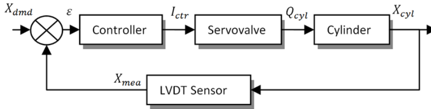
Figure 2: Actuation Loop Scheme. Where X_{dmd} is the position demand, X_{mea} the measured position, \varepsilon the error, I_{ctr} the control current, Q_{cyl} the actuation flow sent to the cylinder and X_{cyl} the real position of the cylinder
