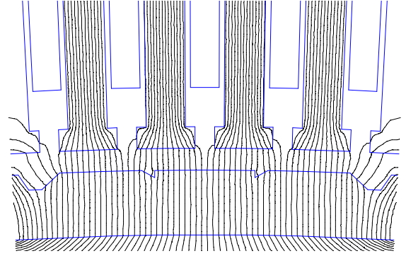
(a) Numerical estimation (FEA program FEMM )
