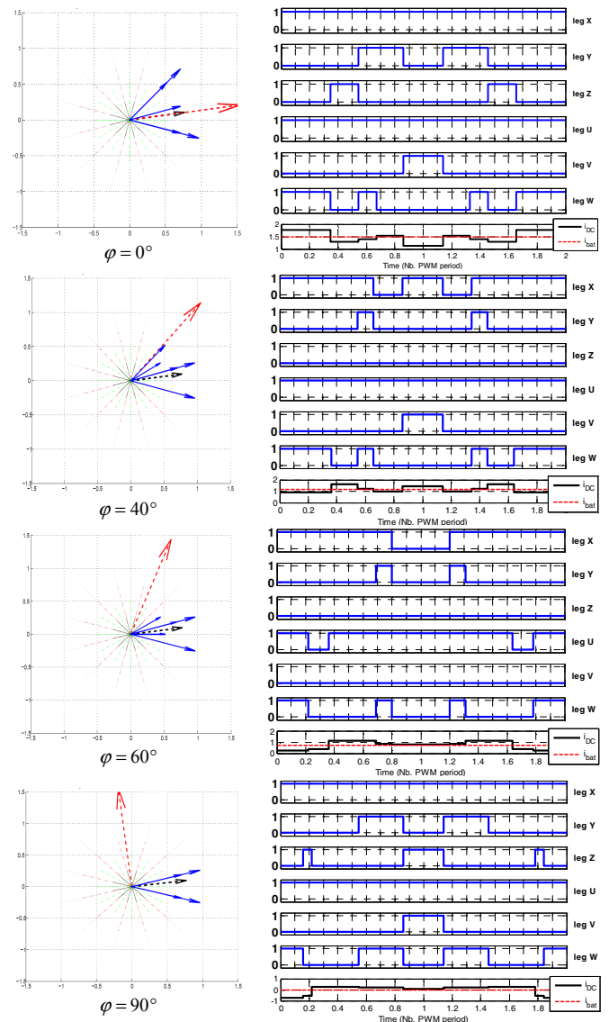
Figure 10: Switching modes selection for each operating point (m=1, \varphi) for 6_DC_RMS_PWM– The black arrow: V_{\alpha\beta}^* , the red arrow: I_{\alpha\beta} and the blue arrows: voltage command vectors
