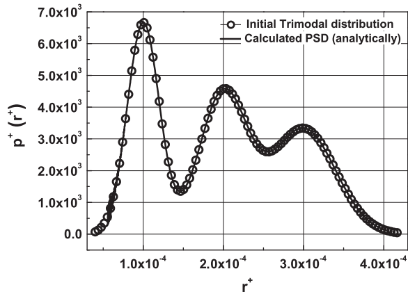
Fig. 14. Comparison between the initial and the calculated PSD for a tri-modal distribution with \mu_2^+ = 2\mu_1^+ , \mu_3^+ = 3\mu_1^+ and \sigma_2^+ = 3\sigma_1^+/2 , \sigma_3^+ = 2\sigma_1^+ for a Casson fluid.
