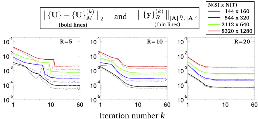
Fig. 9. Influence of discretization parameters on the convergence of the multi-field (IMR) PGD algorithm. Errors are calculated for a fixed decomposition rank M = 10 and the test case \Delta T_{\text{load}} = 0.2 ms.
