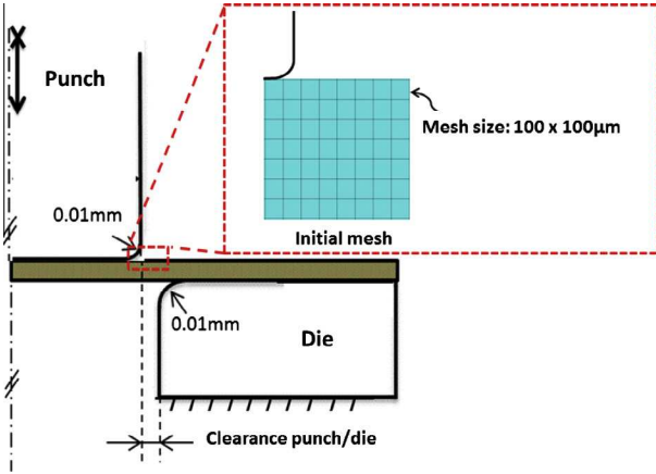
Fig. 5. The boundary conditions and the initial mesh used in the finite element simulations [25].
