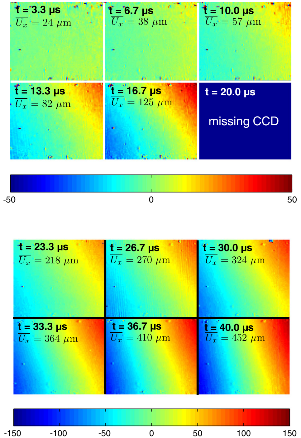
Fig. 15 ( U_x - \overline{U_x} ) maps (colormap in \mu\text{m} ) (test 2, tensile direction: horizontal, field of view: 20 \times 16 mm)
