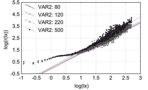
Fig. 14. Evolution of the curvature radius \log(r(l_x)) versus \log l_x for pure Aluminium sheet surface polished with different paper grades 80, 120, 220 and 500 ( l_x and r(l_x) in \mu\text{m} ).
