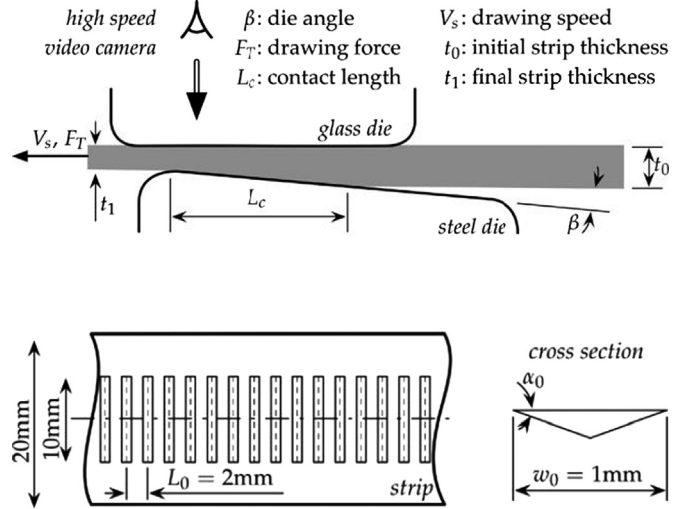
Fig. 6. Schematic diagram of experimental device used for drawing process after [31].
