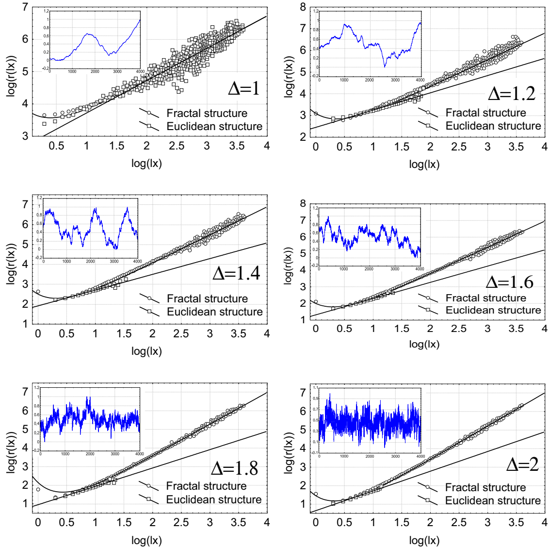
Fig. B2. Evolution of the fractal curvature radius \log(r(l_x)) and Euclidean curvature radius \log(\tilde{r}(l_x)) versus \log(l_x) for different fractional Brownian curves (fractal dimension 1, 1.2, 1.4, 1.6, 1.8, 2) with their associated profiles.
