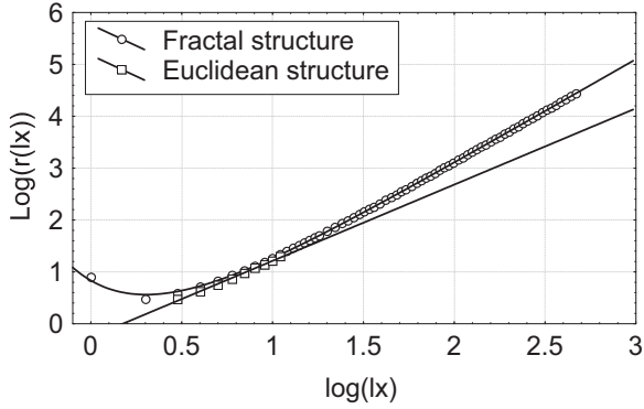
Fig. B1. Evolution of the fractal curvature radius \log(r(l_x)) and Euclidean curvature radius \log(\tilde{r}(l_x)) versus \log(l_x) for a white noise.
