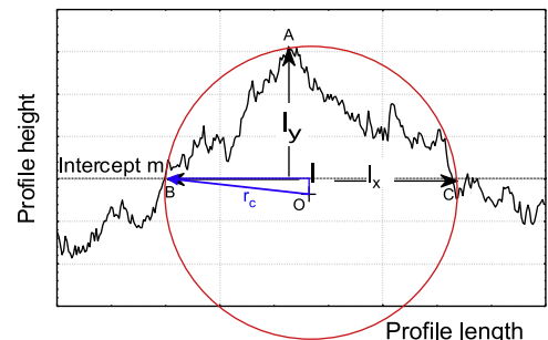
Fig. 1. Definition of l_x and l_y used to calculate the local curvature radius r_c(l_x) .
