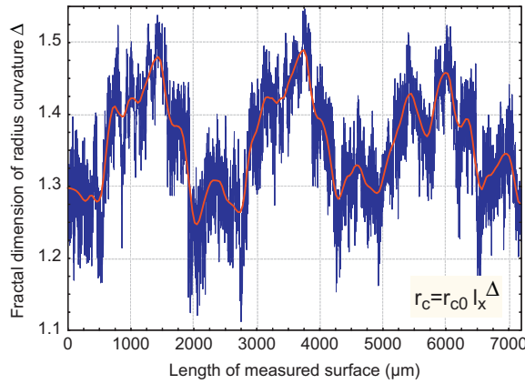
Fig. 12. Evaluation of the fractal dimension \Delta(p) versus the measured surface along the drawing direction p .
