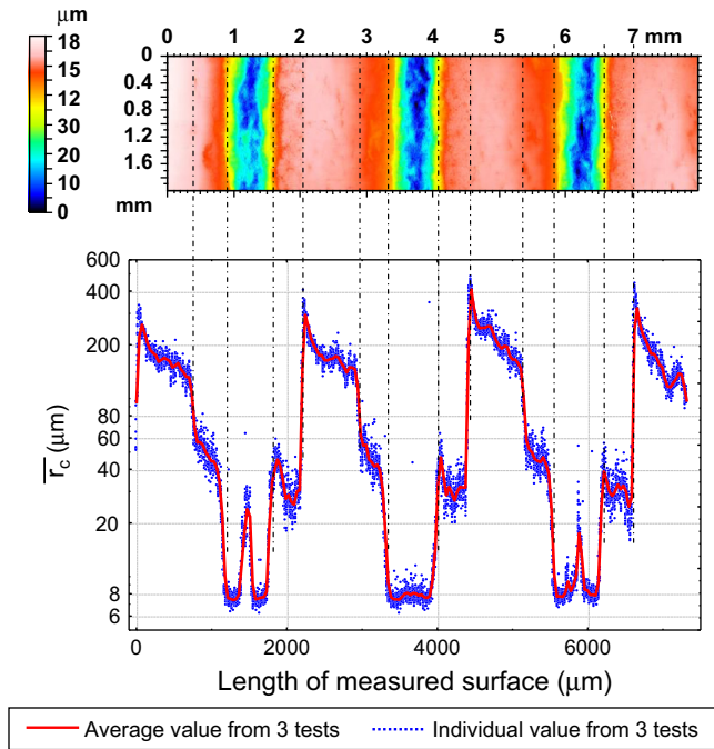
Fig. 10. Analysis of average roughness peaks curvature radius ( \bar{r}_c ) calculated on individual 2D profiles extracted from surface in vertical direction, every point on bottom graphs corresponds to roughness parameter calculated from one vertical profile.
