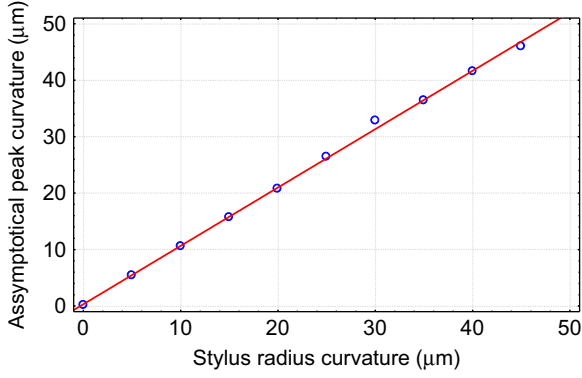
Fig. 18. Plot of the asymptotic peak curvatures of Fig. 17 versus the profiler stylus tip curvature.
