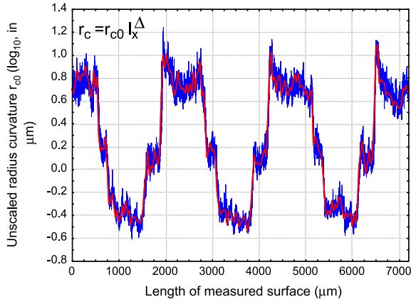
Fig. 11. Evaluation of the unscaled curvature radius r_{c0}(p) versus the measured surface along the drawing direction p .
