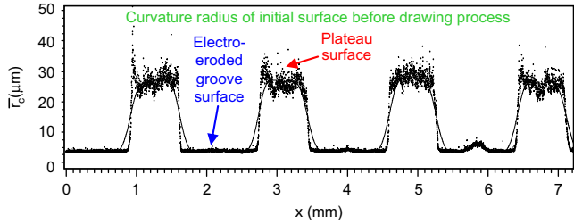
Fig. 9. Averaged curvature of peaks roughness \bar{r}_c calculated on initial profile before drawing process, showing very regular sharp peaks in electroeroded zone (small \bar{r}_c around 6 \mu\text{m} ) and higher peaks value on plateau ( \bar{r}_c around 30 \mu\text{m} ).
