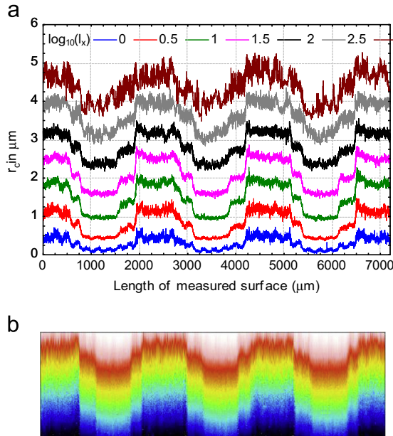
Fig. 13. Multiscale decomposition of r_c(l_x, p) , (a) decomposition graph, (b) decomposition map.
