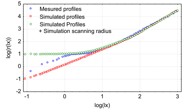
Fig. 16. Evolution of the curvature radius \log r_c(l_x) versus \log l_x for profile shown in Fig. 15a, Fig. 15b and Fig. 15c ( l_x and r(l_x) in \mu\text{m} ).
