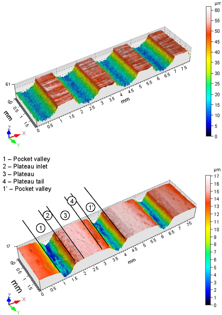
Fig. 7. Initial textured surface with pockets prepared by electro erosion process and final morphology after drawing test, lubricated by mineral oil, different zones created on textured surface can be defined.
