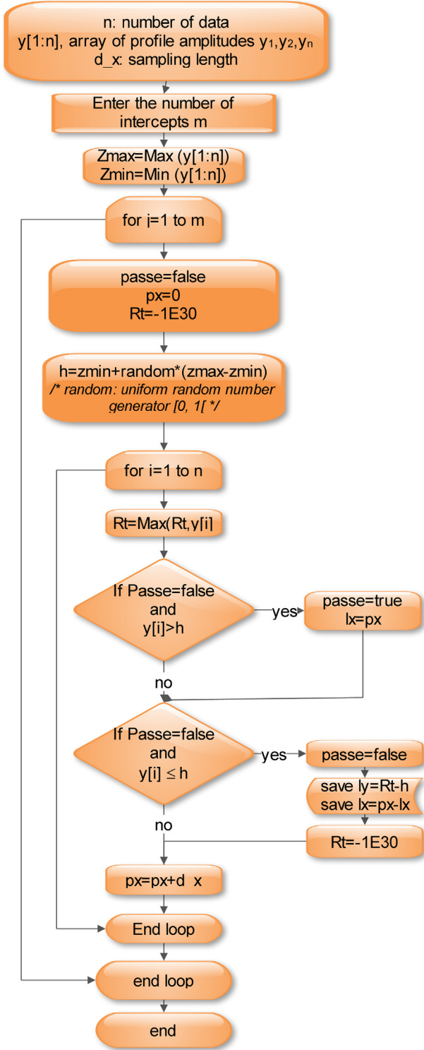
Fig. 2. Algorithm used to calculate the Curvature Radius Estimation on Fractal Surface.
