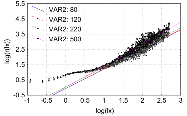
Fig. 14. Evolution of the curvature radius \log r_c(l_x) versus \log l_x for pure Aluminium sheet surface polished with different paper grades 80, 120, 220 and 500 ( l_x and r(l_x) in \mu\text{m} ).
