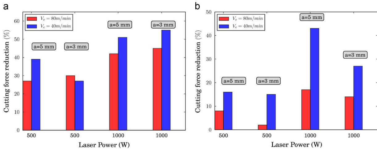
Fig. 10. Cutting force reduction, (a) f=0.1 mm/rev, (b) f=0.2 mm/rev.
