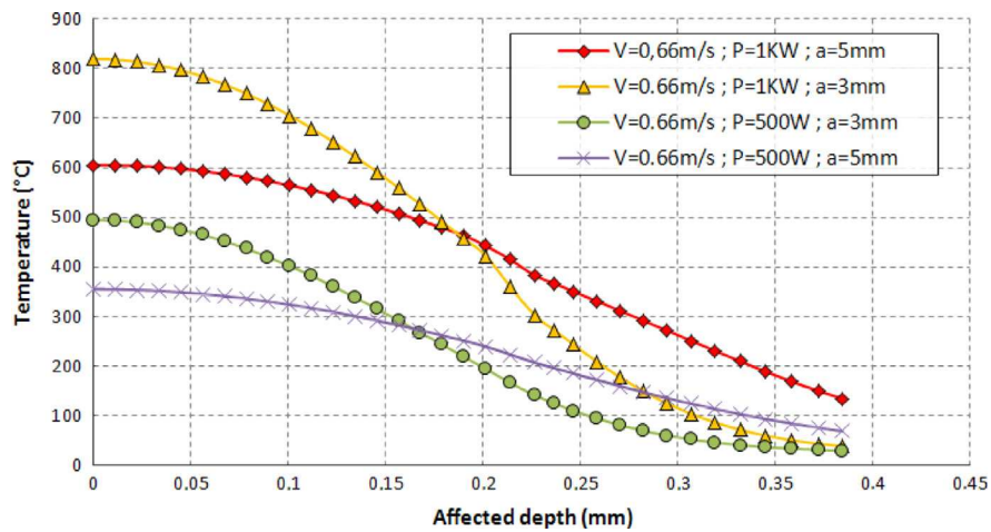
Fig. 4. Affected depth.
