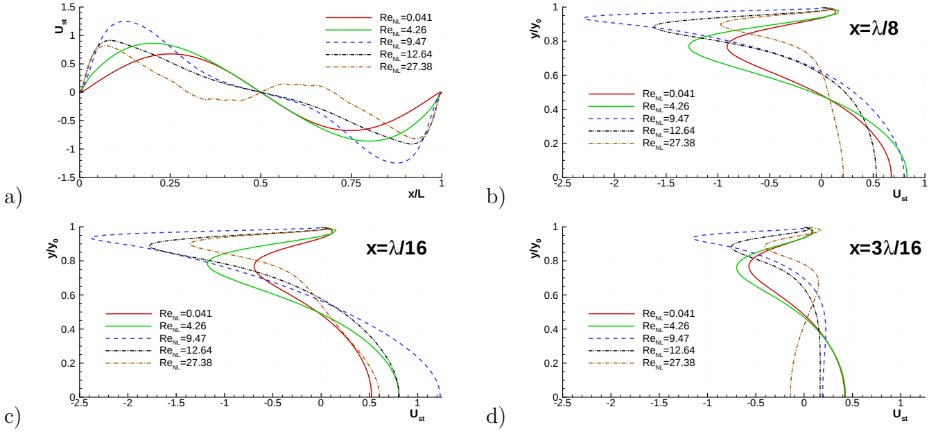
Figure 4: Horizontal mean velocity component U_{st} , normalized with \frac{3}{16} U_{max}^2 / c_0 for the 5 cases of Figure 3. a) U_{st} along the channel's central axis. b), c) and d) U_{st} as a function of y/y_0 for several sections x .
