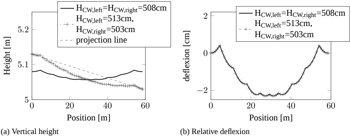
Figure 3: Variation of +5\text{cm} for H_{CW, \text{left}} and -5\text{cm} for H_{CW, \text{right}}
