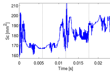
Figure 11: Effective (or closed) contact area as function of time for the cycle of maximal amplitude.
