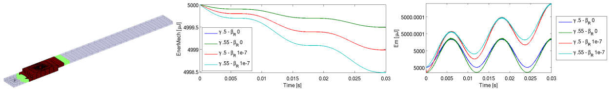
Figure 5: Left: the kept area chosen for the lap-joint model (in red), reduced part (in blue) and reduced coupling element layer (in green). Middle: Effect of numerical damping on the mechanical energy evolution (linear case). Right: Mechanical energy with scheme compensation (linear case)
