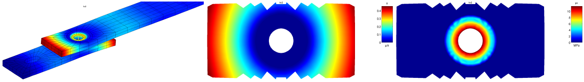
Figure 4: Static bolt pre-stress, deformation field, gap (max 0.4\mu m ) and pressure fields (max 15MPa )
