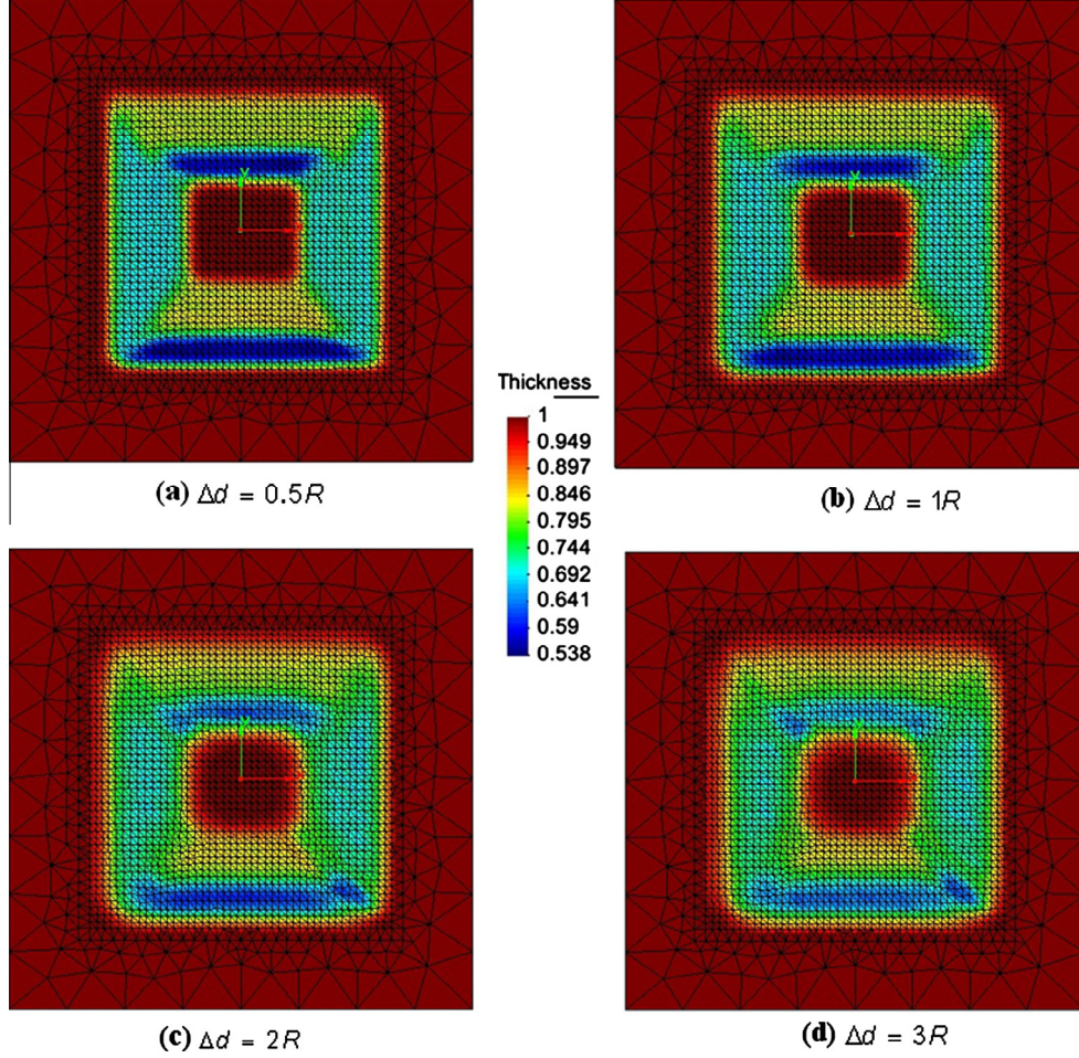
Fig. 11. Thickness distributions.
