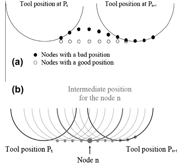
Fig. 9. Tool position strategy.
