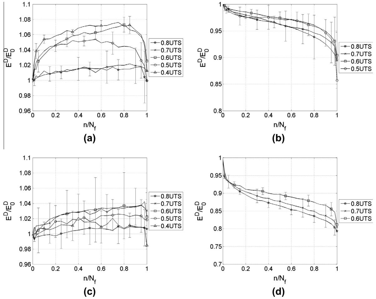
Fig. 8. Evolution of the normalized dynamic modulus for (a) FE_0, (b) FE_90, (c) FE_090 and (d) FE_45 for loading levels from 0.4 to 0.8 UTS.
