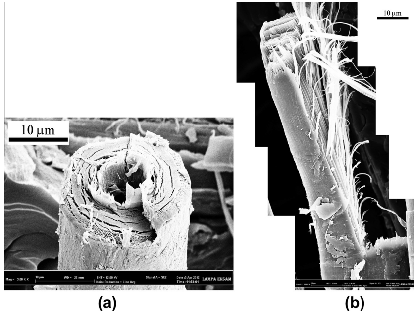
Fig. 9. SEM view of (a) the concentric structure of flax fibre with presence of lumen and (b) longitudinal view of broken fibre with pull-out of microfibrils.
