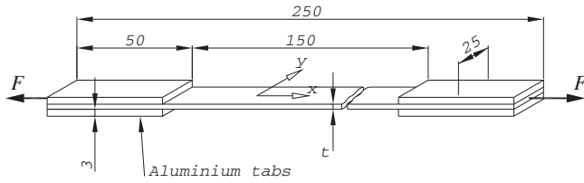
Fig. 1. Geometry of the fatigue specimens. Dimensions in mm. The x and y axes were designated as the longitudinal and transverse in-plane directions respectively.
