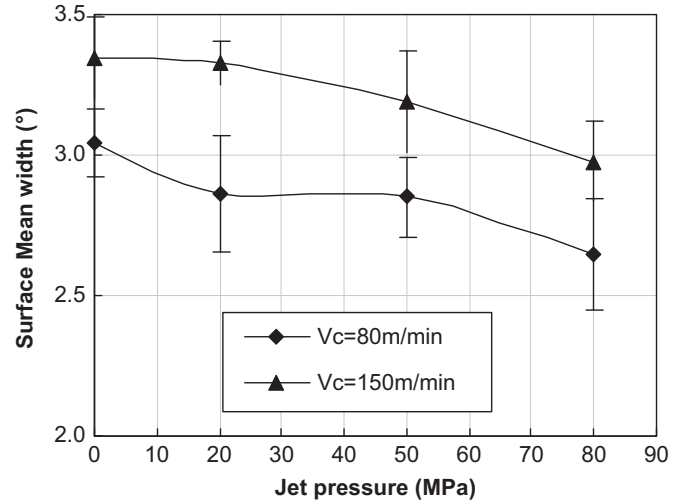
Fig. 13. Evolution of the surface mean X-ray diffraction peak width as a function of the jet pressure ( V_c=80 and 150 \text{ m/min} , f=0.1 \text{ mm/rev} and a_p=1 \text{ mm} ).
