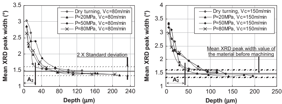
Fig. 12. Mean X-ray diffraction peak width profiles obtained by using dry and HPWJAT ( f=0.1 \text{ mm/rev} and a_p=1 \text{ mm} ).
