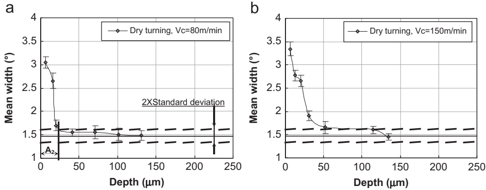
Fig. 11. Mean X-ray diffraction peak width profiles obtained by dry turning: (a) V_c=80 \text{ m/min} and (b) V_c=150 \text{ m/min} .
