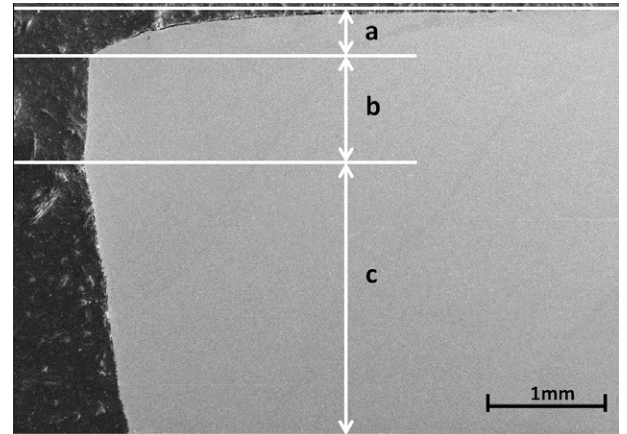
Fig. 7. Experimental shearing profile.
