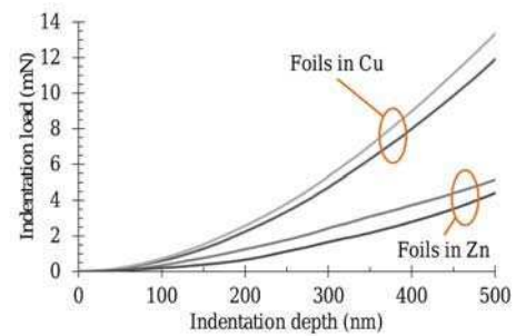
Fig. 6. Indentation load-depth curves for foils in copper and zinc obtained by S.I.P
