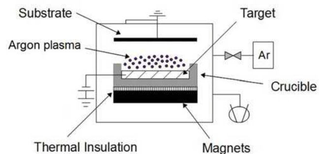
Fig. 1. Sketch of the self-induced ion plating (S.I.P) process
