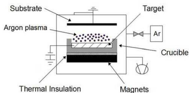
Fig. 1. Sketch of the self-induced ion plating (S.I.P) process
