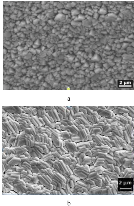
Fig. 5. Illustration of copper foil microstructures obtained by varying process parameters (SEM observations)
