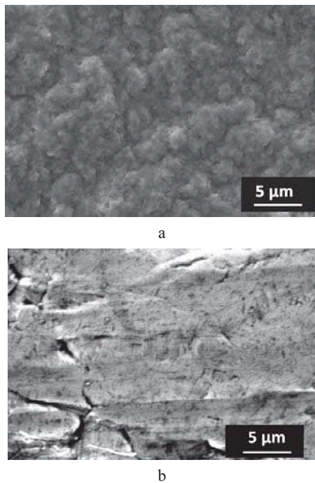
Fig. 7. SEM observations of the microstructure of: copper foils obtained by electroplating (a) and zinc foils obtained by rolling (b)
