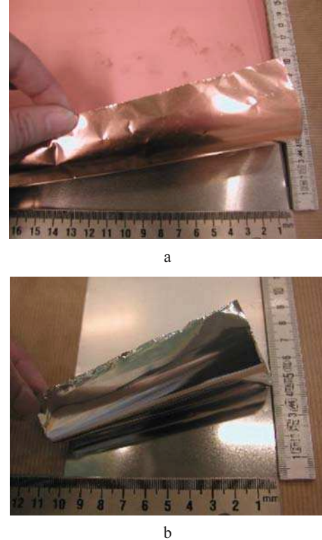
Fig. 3. Foil in copper (a) and in zinc (b) obtained by vacuum deposition on steel
