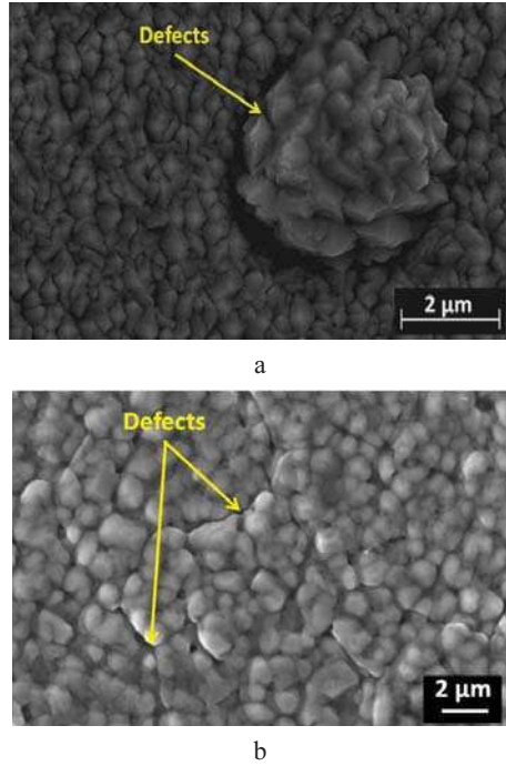
Fig. 4. SEM observations of the microstructure of copper (a) and zinc (b) foils obtained by vacuum deposition
