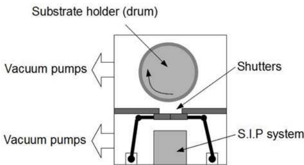
Fig. 2. Sketch of the semi-industrial pilot used for the deposition by S.I.P
