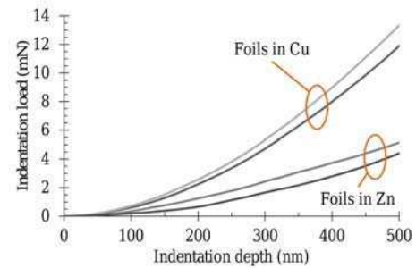
Fig. 6. Indentation load-depth curves for foils in copper and in zinc obtained by S.I.P
