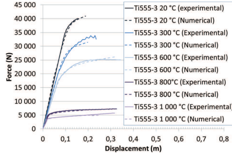
Fig. 11 Comparison between the experimental and numerical force-displacement curves at different temperature for the Johnson–Cook model identified for Ti555-3 alloy (strain rate = 1 s^{-1} )
