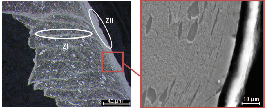
Fig. 12 Observation of white bands in ZI and ZII (Ti555-3, tool CP500, V_c = 90 m/min, f = 0.15 mm/rev)
