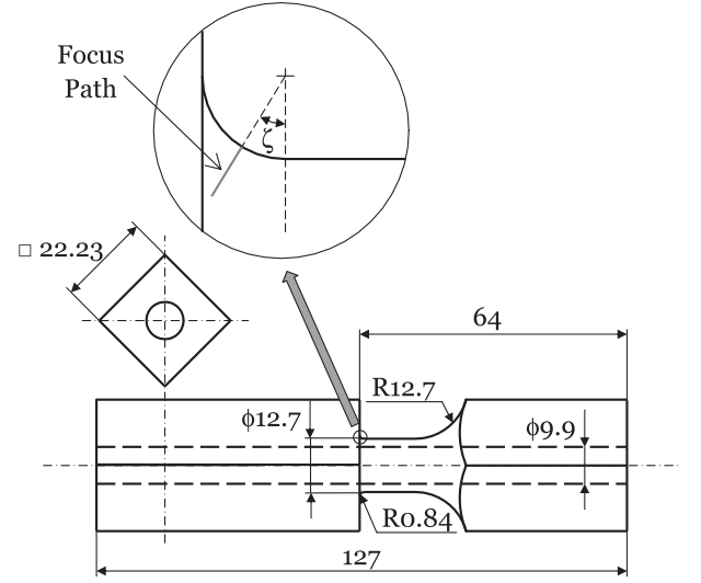
Fig. 3. Specimens with fillet of steel S65A tested by Gough [6] and angle \zeta defining the orientation of the focus path.
