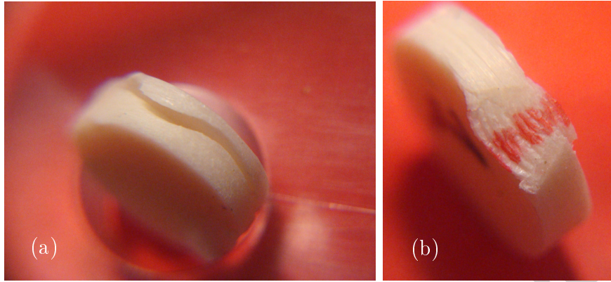
Figure 6: Examples of abnormal splitting due to shear stress (a) and matting (b).
