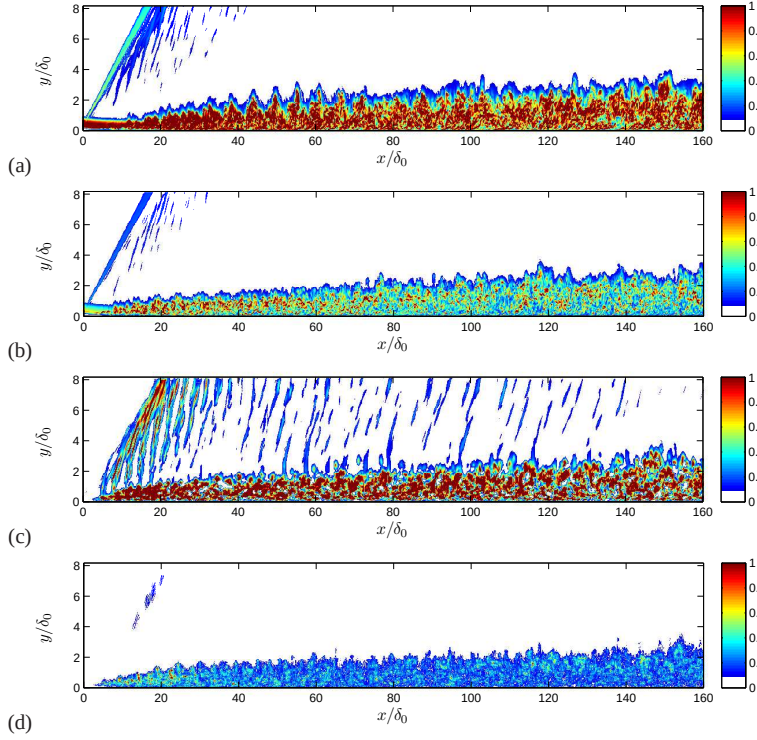
Fig. 14 Influence of the SGS model for the supersonic boundary layer. Colormaps of instantaneous normalized eddy viscosity v_t/v (levels between 0 and 1); (a) SM with C_S=0.15 ; (b) SM with C_S=0.1 ; (c) DSM; (d) MSM-ss. \delta_0 is the initial boundary layer thickness.
