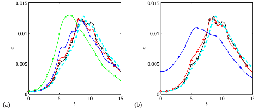
Fig. 5 Influence of the RT methodology filter stencil for the Taylor-Green vortex. (a) For standard filters. Kinetic energy dissipation \varepsilon for: (—□—) 4 th -order; (—*—) 6 th -order; (—△—) 8 th -order; (—○—) 10 th -order. (b) For optimised filters. Kinetic energy dissipation \varepsilon for: (—*—) 7-point DRP filter ([35]); (—△—) 9-point DRP filter ([35]); (—○—) 11-point DRP filter ([36]); (— —) 256^3 (see Fig.3).
