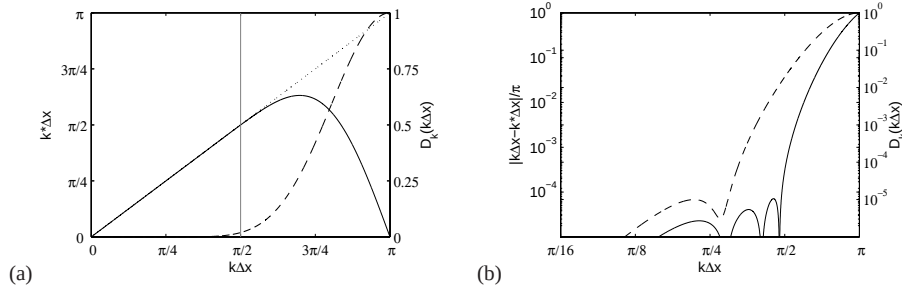
Fig. 1 Fourier analyses of central finite-difference and filter schemes. (a) The effective wavenumber k^*\Delta x of the 11-point finite-difference scheme (—) and the damping function D_k(k\Delta x) of the 11-point filter (---) are plotted as function of the reduced wavenumber k\Delta x with scales on the left and on the right, respectively. The dotted line represents the exact relationship for the discretization scheme and the vertical gray line marks the limit of resolvability k\Delta x \approx \pi/2 . (b) Logarithmic scales are proposed for the dispersion error of finite differences (—) with scale on the left axis and for the dissipation error of the filter (---) with scale on the right axis.
