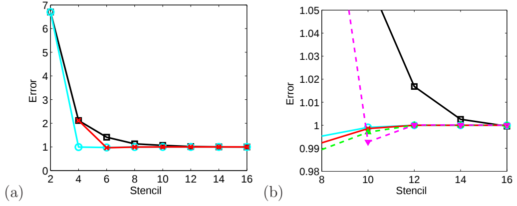
Figure 21: Normalized error at the final iteration for the 1-D advection of a wavepacket as a function of the size N of the interpolation stencil. (a) Lagrange interpolations (—□), fully optimized interpolations (—○), and optimized interpolation with fourth order constraint (—×); (b) close-up view for large stencils. Two methods for the evaluation of interpolation coefficient are added: optimized interpolation with sixth-order constraint (—△), and with eighth-order constraint (—▽).
