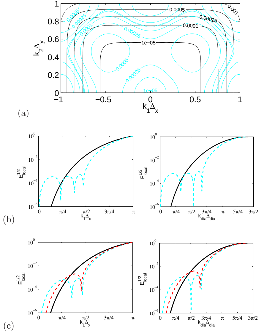
Figure 17: Optimized 2×1D interpolation with or without order constraints. (a) Map of the two-dimensional local error for an optimized 2×1-D interpolation (—), superimposed on the reference error using the polar mapping (—). (b) Profiles of the error along k_1\Delta_x (left) and along k_1\Delta_x = k_2\Delta_y (right) for the fully optimized 2×1-D interpolation (---). (c) Same profiles for the optimized 2×1-D interpolation with fourth-order (---) or sixth-order (---) constraint.
