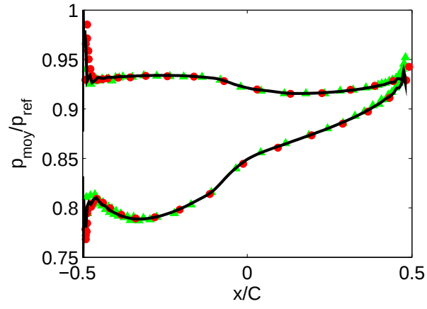
Figure 32: Mean pressure loading on the vane: present overset computation (—), code Turbo , Envia [45] (•), Nallasamy et al. [43] (▲).
