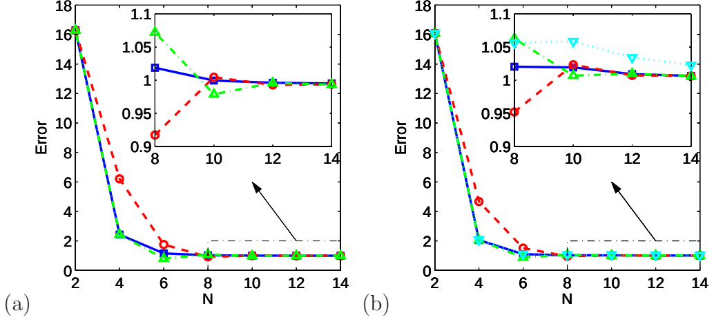
Figure 25: Advection of a vortex. Normalized error on the pressure between the numerical and analytical solutions at the last iteration with a stencil N \times N , for Lagrange interpolations ( \text{---}\square ), fully optimized interpolations ( \text{---}\text{---}\circ ), and optimized interpolations with 4 th -order constraint ( \text{--}\cdot\text{--}\cdot\triangle ). (a) foreground Cartesian grid, (b) foreground sinusoidal grid. The inserts show close-up for large stencils. For the sinusoidal grid (b), the effect of turning off the high-order evaluation of the offsets with the isoparametric mapping is shown ( \cdots\triangledown ).
