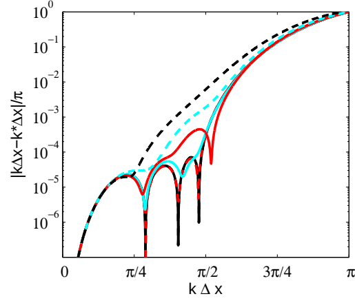
Figure 8: Dispersion error of a scheme combining an eleven-point derivative and q interpolations: q = 1 ( - - - ), q = 2 ( — ), q = 3 ( — ), q = 4 ( - - - ), q = 5 ( - - - ). Dispersion error of the finite-difference derivative alone ( — ) is plotted as a reference. Lagrange interpolations are used with a stencil of size N = 8 .
