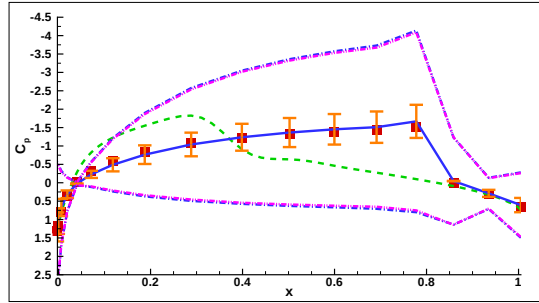
Figure 24: Martin-Hou - C_p vs x . Solutions: reference (■), nominal (— — —), a posteriori (—). Error bars (three times the standard deviation): experimental (—). Error ranges (three times the standard deviation): parametric + model-inadequacy (— — —), model (— · —).
