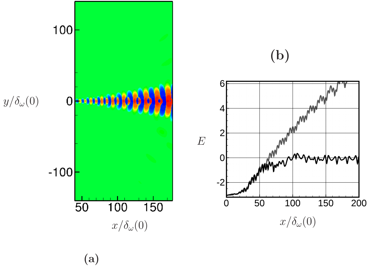
FIG. 9. LDE simulation for the subsonic case; (a) the pressure field is shown; (b) integrated energy associated with disturbances for NLDE(—) and LDE (—) simulations are plotted in a logarithmic scale.
