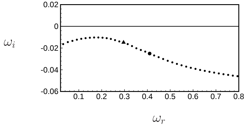
FIG. 23. Global spectrum of the supersonic mixing layer. The eigenvalues are made dimensionless by \delta_\omega(0) and U_c .
