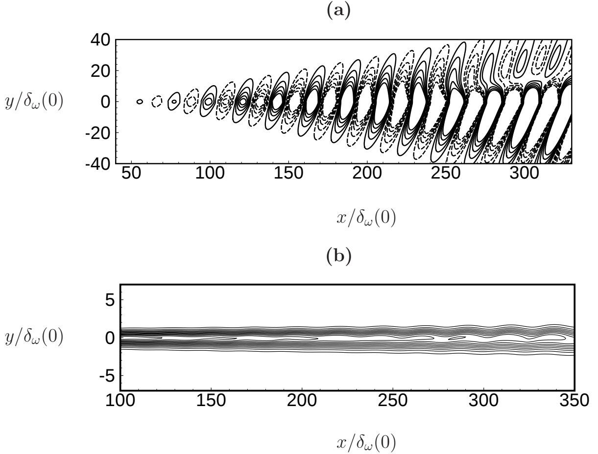
FIG. 21. (a) Far-field non-dimensional fluctuating pressure field with contours levels from -0.01 to 0.01 in steps of 0.002 (full lines: positive values, dashed lines: negatives values). (b) Total non-dimensional spanwise vorticity with contours ranging from 0.05 to 1.5 in steps of 0.05 .
