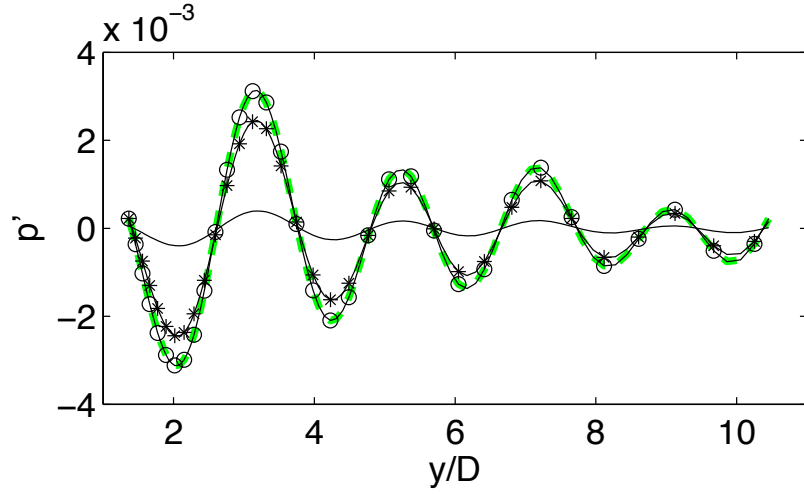
Figure 7: Fluctuating estimated QSE pressure from POD modes 3 & 4 along the line x/D=0.088 for different reference points: (—○—○—○—○—) 4 points located at (1.89; 0.01), (0.34; 0.01), (1.89; -0.72), (0.34; -0.72); (—○—○—) 1 point at (1.89; 0.01); (—*—*) 1 point at (0.34; 0.01); (—) 1 point at (0.34; -0.72).
