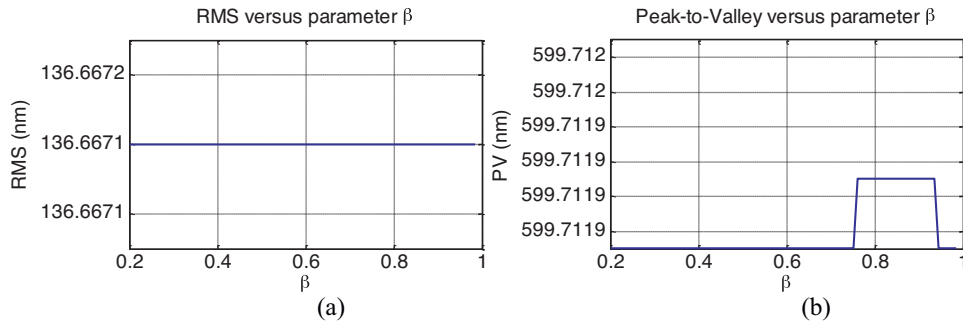
Fig. 11. The influence of \beta on the residuals for the simulated combined errors dataset. (a) RMS residuals; (b) PV residuals.
