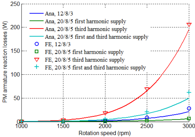
Fig. 8. Armature reaction PM losses.
