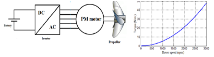
Fig. 1. Chain of electrical naval propulsion.
