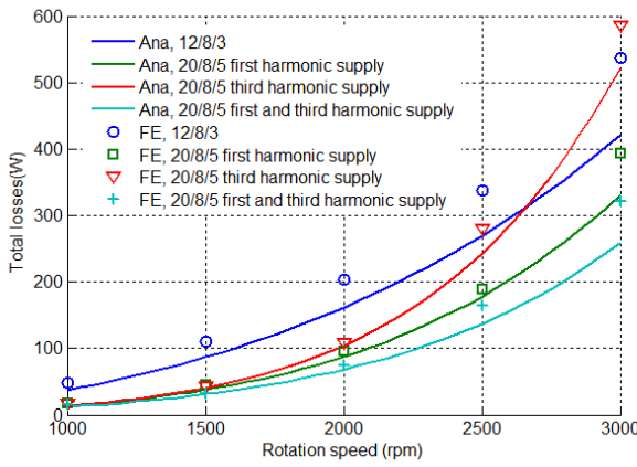
Fig. 11. Total losses in the two machines.
