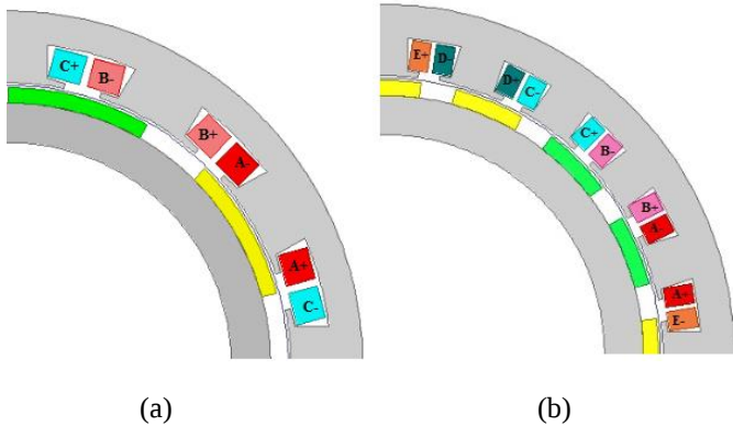
Fig. 4. (a) 12/8/3 machine . (b) 20/8/5 machine.
