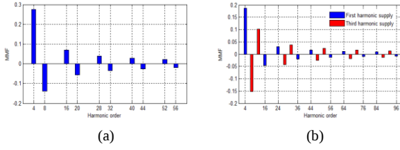
Fig. 7. MMF spectrum .(a) 12/8/3 machine ; (b) 20/8/5 machine.
