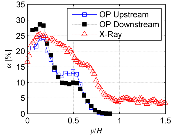
Fig. 20. Comparison of the percent void fraction measured near the cavity closure at x = 5H using x-ray and optical probes data. Data are for q = 4.60 \times 10^{-3} . The error bars for the optical probe data were shown in figure 15b and were O(2\%) . For the x-ray data the standard deviation of the mean in the region of interest was at most 0.74% and had an average of 0.26%. However, the actual uncertainty of the x-ray data is determined by the numerous factors discussed in the text. Most notably, the cavity closure was to a degree three dimensional, and due to the high void fraction gradient the effect of non-parallel beam paths was more significant. As the data available do not allow for good assessment of error due to the 3D nature of the cavity closure, the x-ray error bars are not included.
