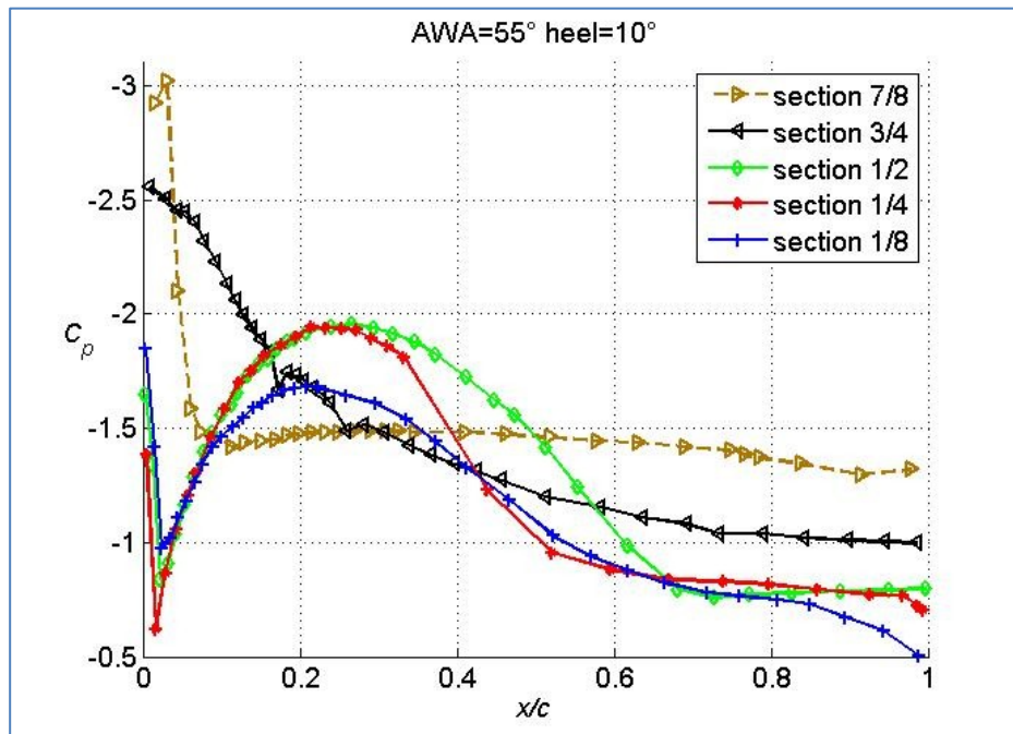
Figure 3: C_p on the 5 sections of the spinnaker for 55° AWA and 10° heel (colours available in the on-line version of the manuscript).
