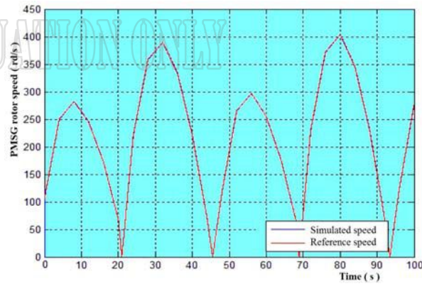
Fig. 11: The PMSG rotor speed and its reference
