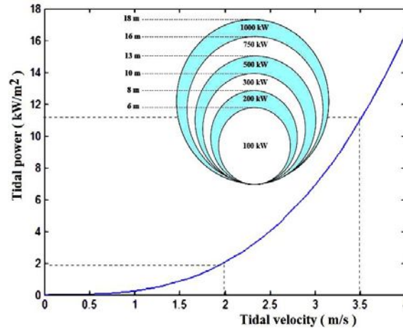
Fig. 3: The harnessed tidal power and power ratings versus the turbine diameter
