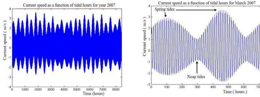
Fig. 4: Tidal velocity in the Raz de Sein for the year 2007 and March 2007
