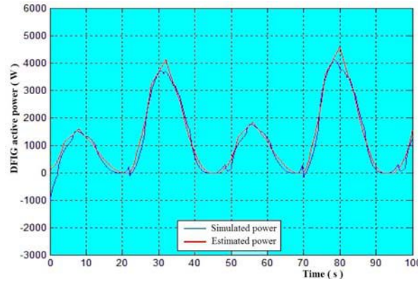
Fig. 10: The DFIG active power
