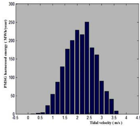
Fig. 15: PMSG-based MCT harnessed energy histogram in one year
