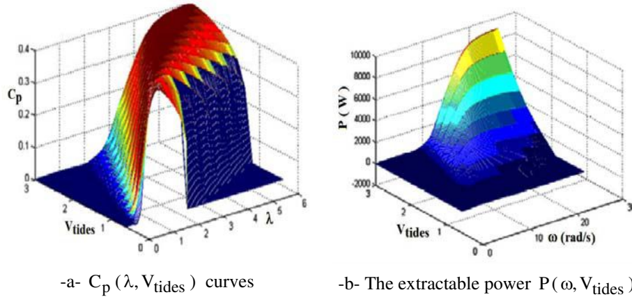
Fig. 5: Calculated hydrodynamics performance of a 1.44 m diameter turbine.
