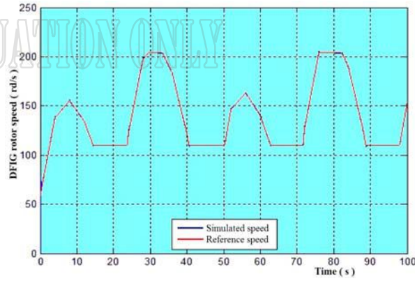
Fig. 9: The DFIG rotor speed and its reference
