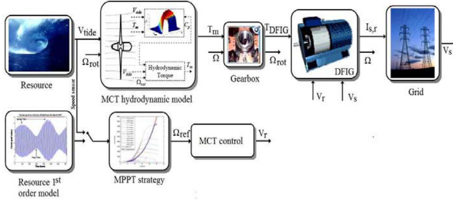
Fig. 8: Variable speed control for a DFIG-based MCT
