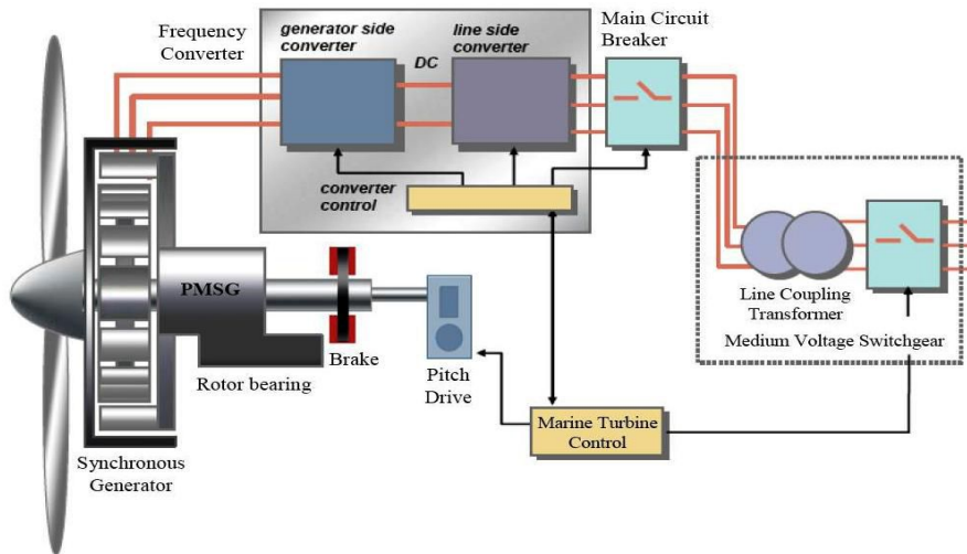
Fig. 7: Schematic diagram of a PMSG-based generation system
