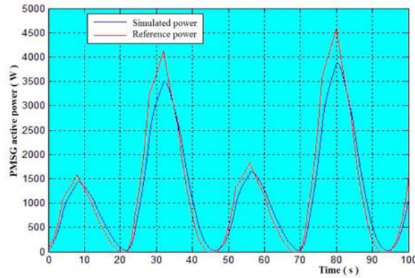
Fig. 12: The PMSG active power
