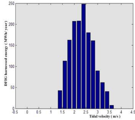
Fig. 14: DFIG-based MCT harnessed energy histogram in one year
