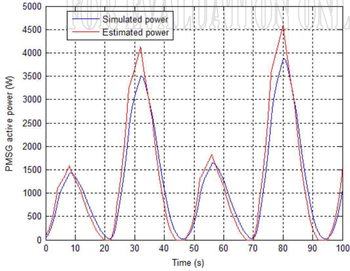
Fig. 11. PMSG active power.
