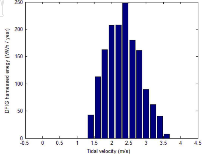
Fig. 18. DFIG-based MCT harnesses energy histogram in one year.
