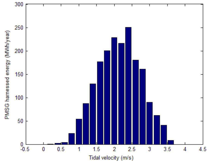
Fig. 19. PMSG-based MCT harnesses energy histogram in one year.
