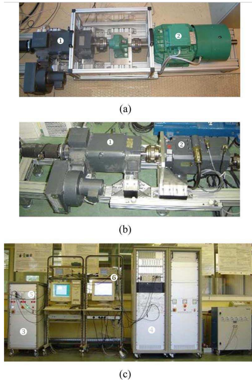
Fig. 12. The experimental setup emulating a marine current turbine [© G2ELAB Grenoble, France]: (a) ① DC motor, ② DFIG; (b) ① DC motor, ② PMSG; and (c) ③ power electronics for driving the DC motor, ④ power electronics for driving the DFIG and the PMSG, ⑤ DSP TMS320F240 implementing DC motor control, ⑥ DSP DS1005 (dSPACE) implementing DFIG- and PMSG-based MCT controls.
