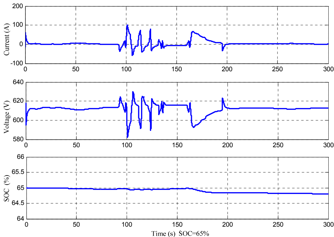
Figure 16. Battery characteristics for Case 2.
