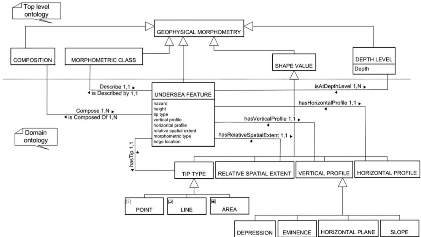
Figure 3. Conceptual model of the submarine relief 6
