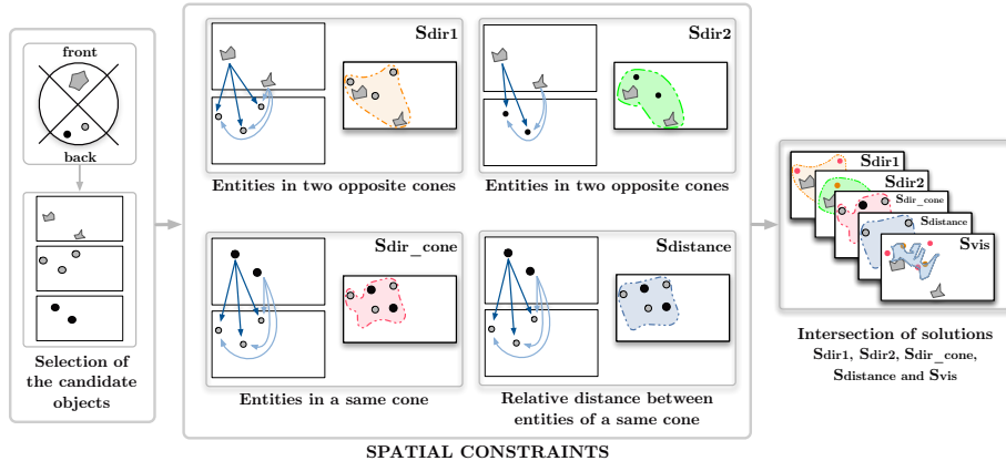
Fig. 9. Constraint-based approach
