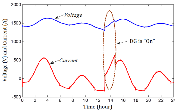
Fig. 15. BESS voltage and current.
