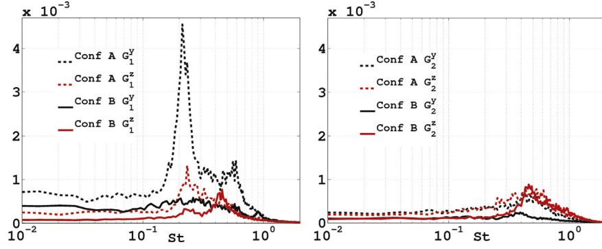
Fig. 5. PSD of the F_1 load (left-hand side) and of F_2 (right-hand side), projected onto z -axis (red color) and onto y -axis (black color). Dashed lines are for configuration A and the filled line for configuration B . These curves are voluntarily set with the same arbitrary units. (For interpretation of the references to color in this figure, the reader is referred to the web version of this article.)
