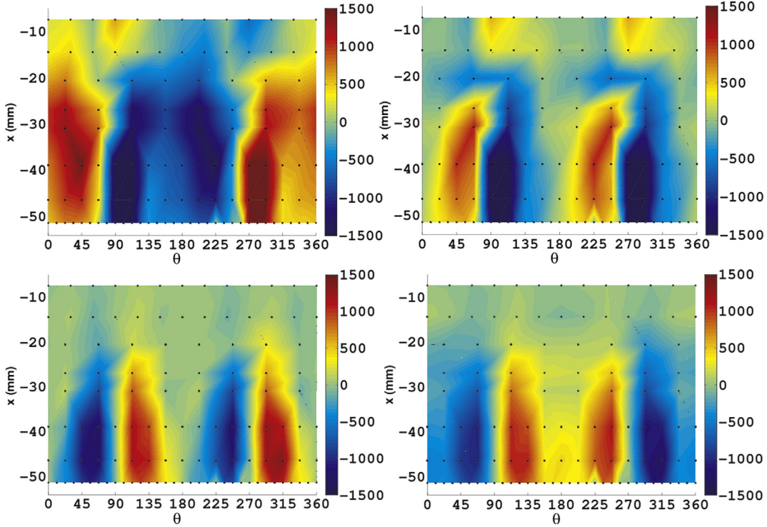
Fig. 7. First (left) and second (right) POD modes of the pressure. Configuration A (top) and configuration B (bottom).
