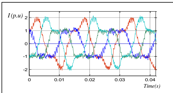
Fig. 9. Experimental results: Optimal currents of machine for single open circuited phase.
