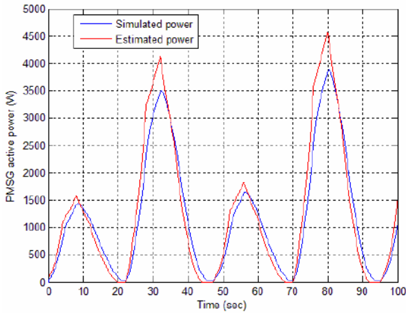
Fig. 12. The PMSG active power.
