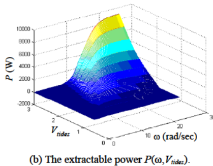
Fig. 5. Calculated hydrodynamics performance of a 1.44 m diameter turbine.
