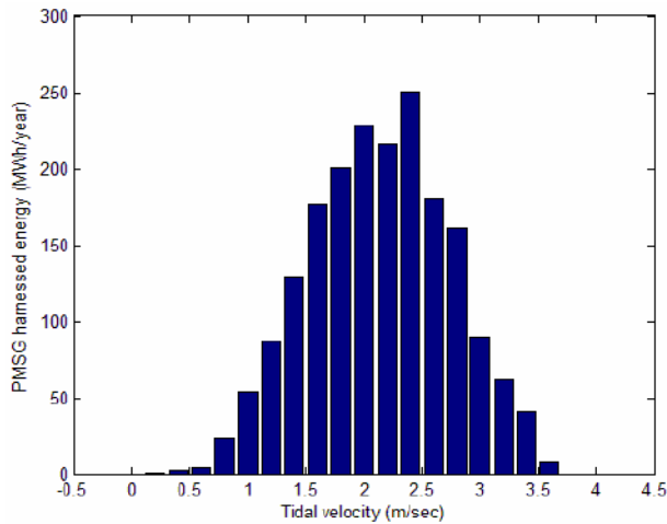
Fig. 15. PMSG-based MCT harnesses energy histogram in one year.
