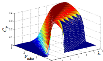
(a) C_p(\lambda, V_{tides}) curves.
