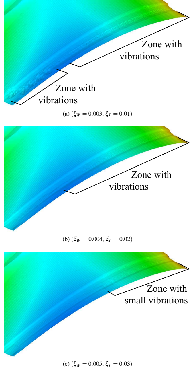
FIGURE 12: TOOL AND WORKPIECE BOTH FLEXIBLE, 10+2 MODES.
