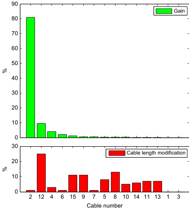
Fig. 9. Percentage length modification (lower panel) and individual percentage reduction attributed to each cable appearing by its contribution to total economy gain. Notice that cable # 2 provides the largest part to total gain.
