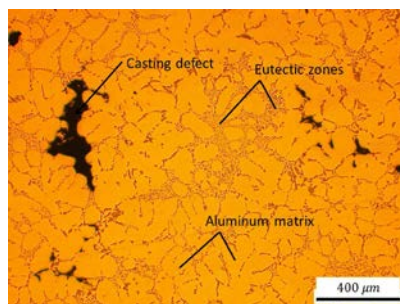
Figure 1: Typical microstructure of a cast Al-Si alloy
