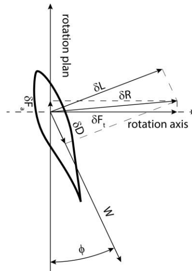
Fig. 4. Aerodynamic forces
